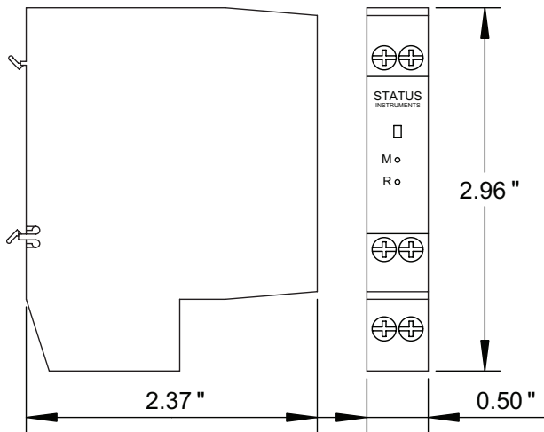
PHYSICAL DIMENSIONS
